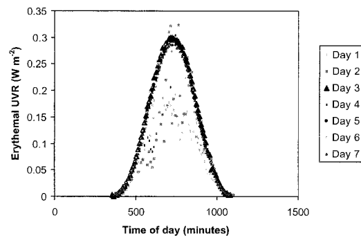
Figure 2. Diurnal variation in ambient erythemal UVR ( W\cdot m^{-2} ) as recorded by the YES UVB pyranometer in Durban for each day of the study period.
