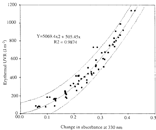
Figure 1. Dose–response calibration curves for PSF showing \Delta A_{330} of PSF versus the YES UVB pyranometer erythemal UV dose, showing the measure of uncertainty with a 95% confidence band.
